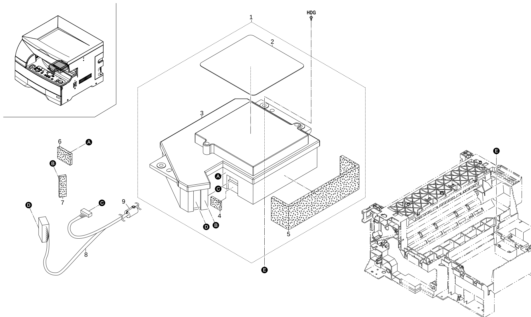
FIG. 7 LASER SCANNER UNIT
