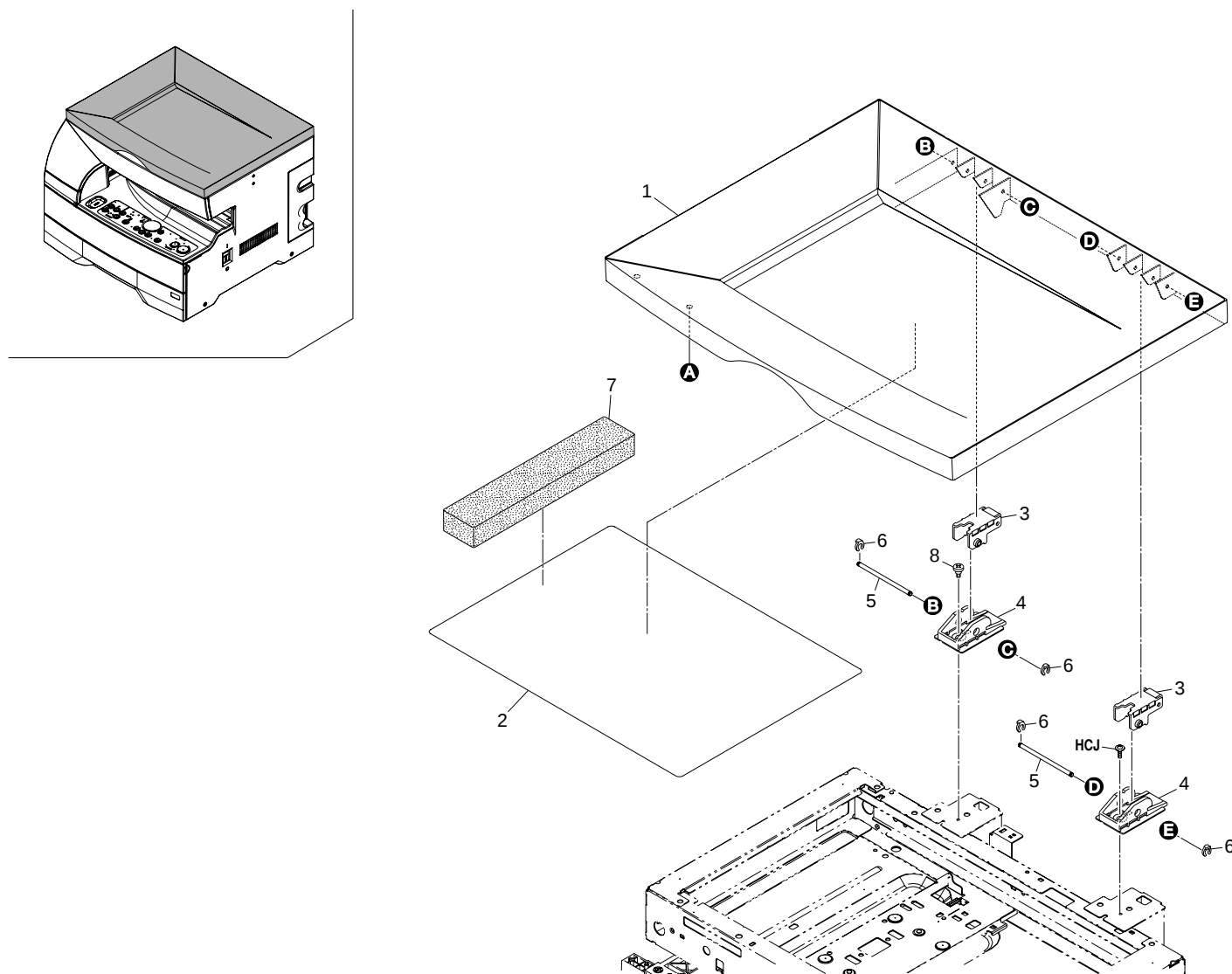
FIG. 5 ORIGINAL HOLDER
