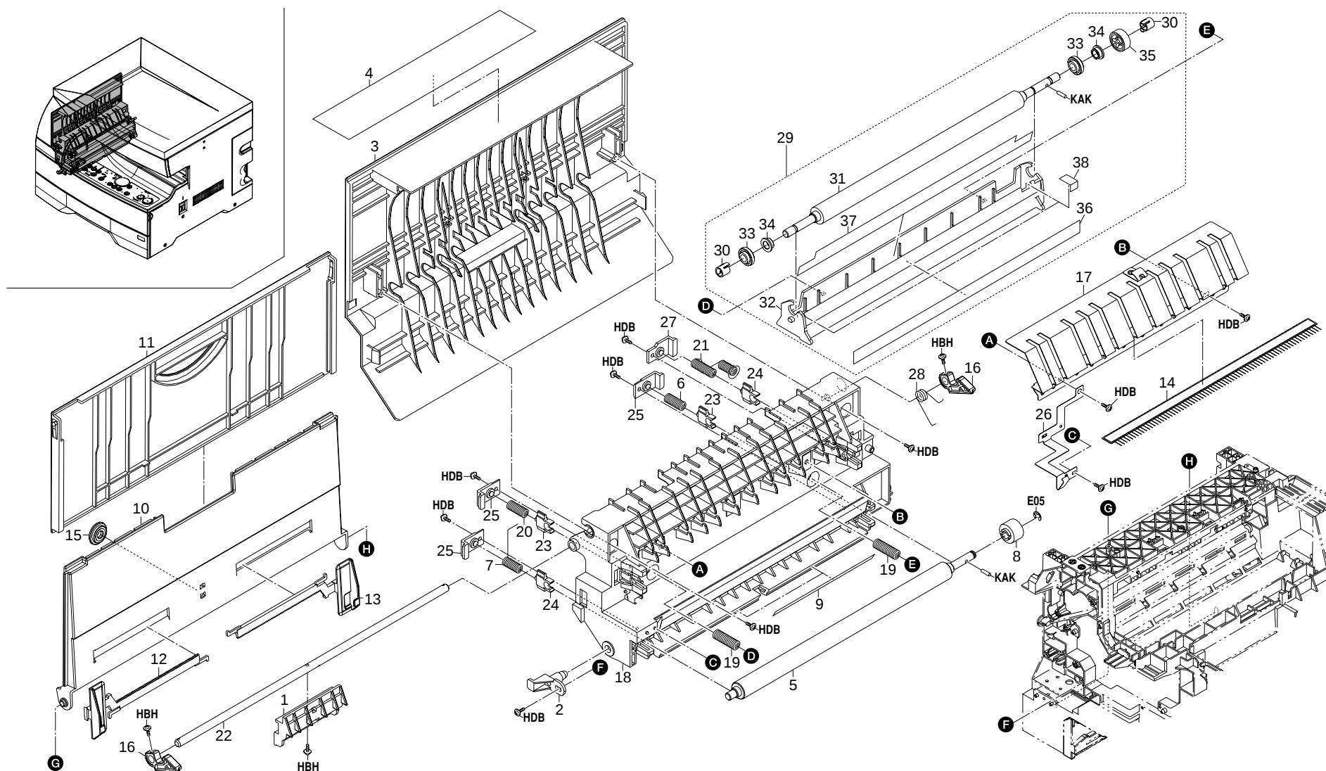
FIG. 4 CONVEYING SECTION
