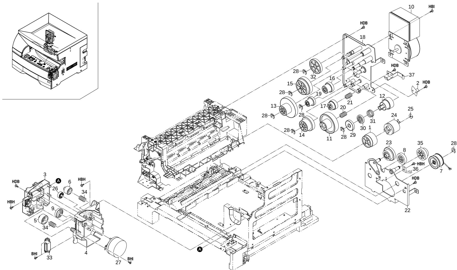
FIG. 11 DRIVING SECTION
