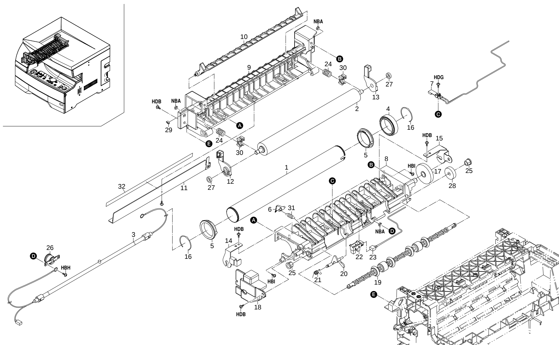
FIG. 10 FIXING SECTION
