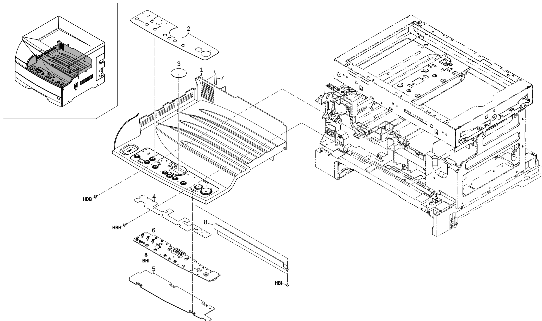
FIG. 13 OPERATION UNIT
