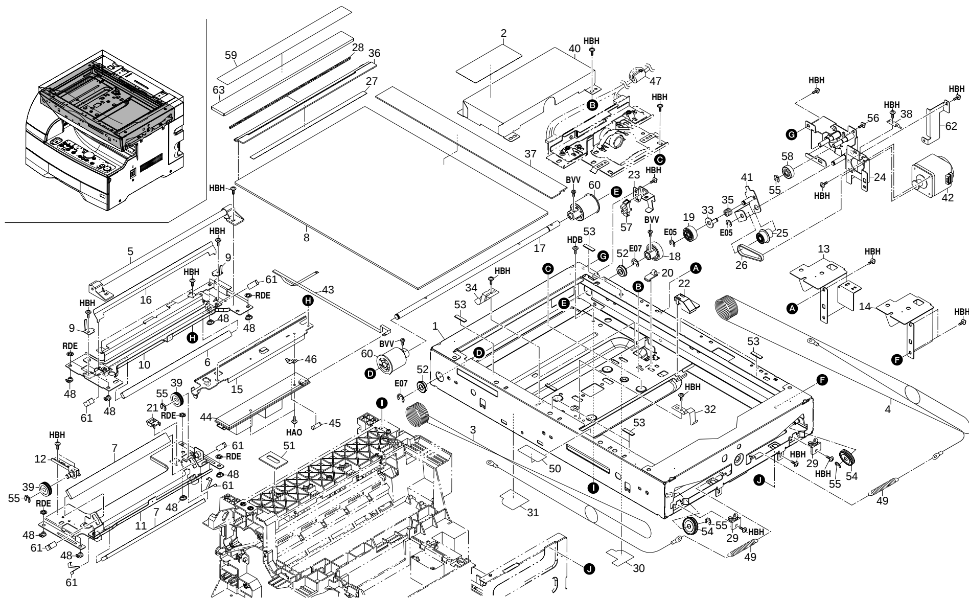
FIG. 6 OPTICAL SECTION
