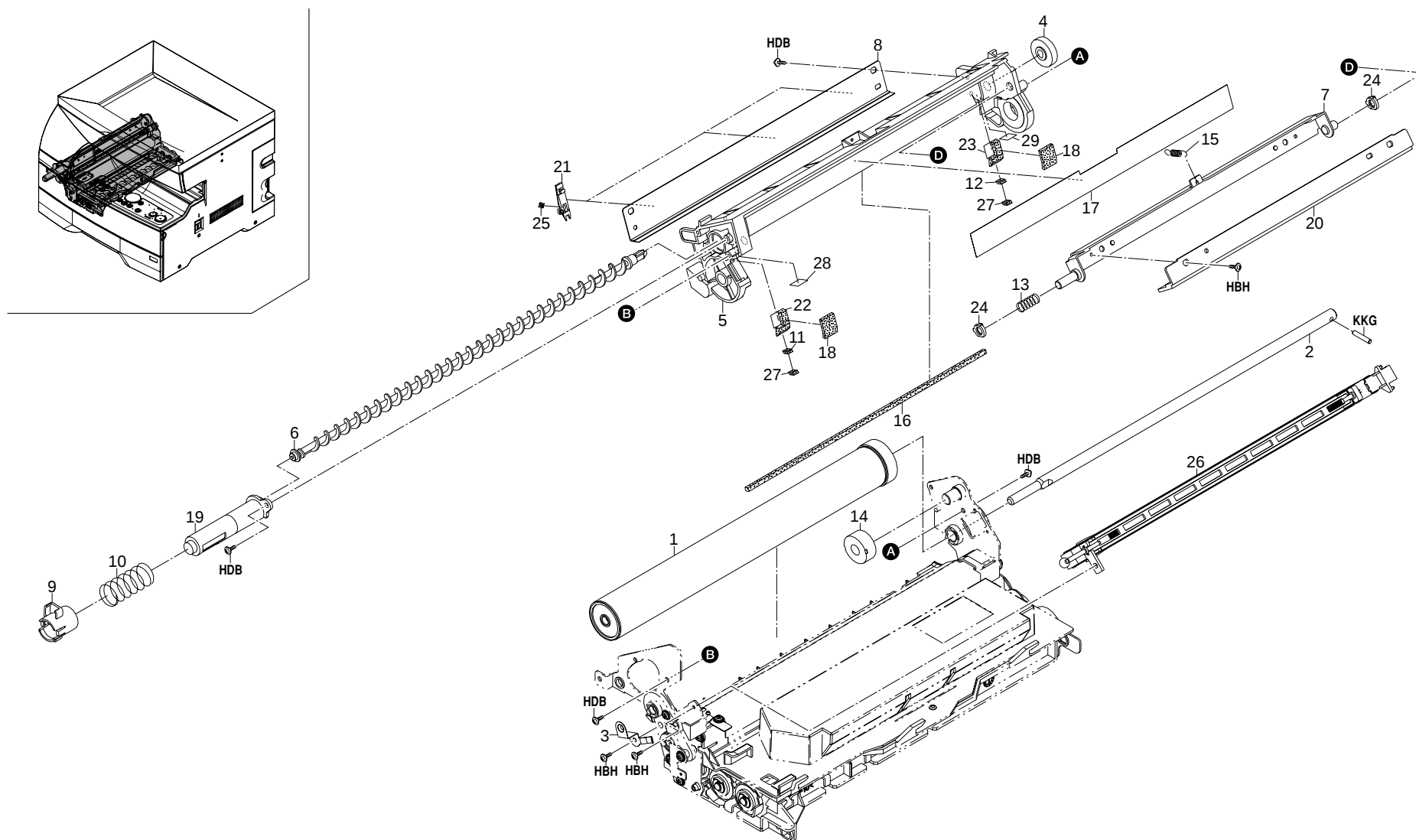
FIG. 9 IMAGING UNIT (CLEANING SECTION)
