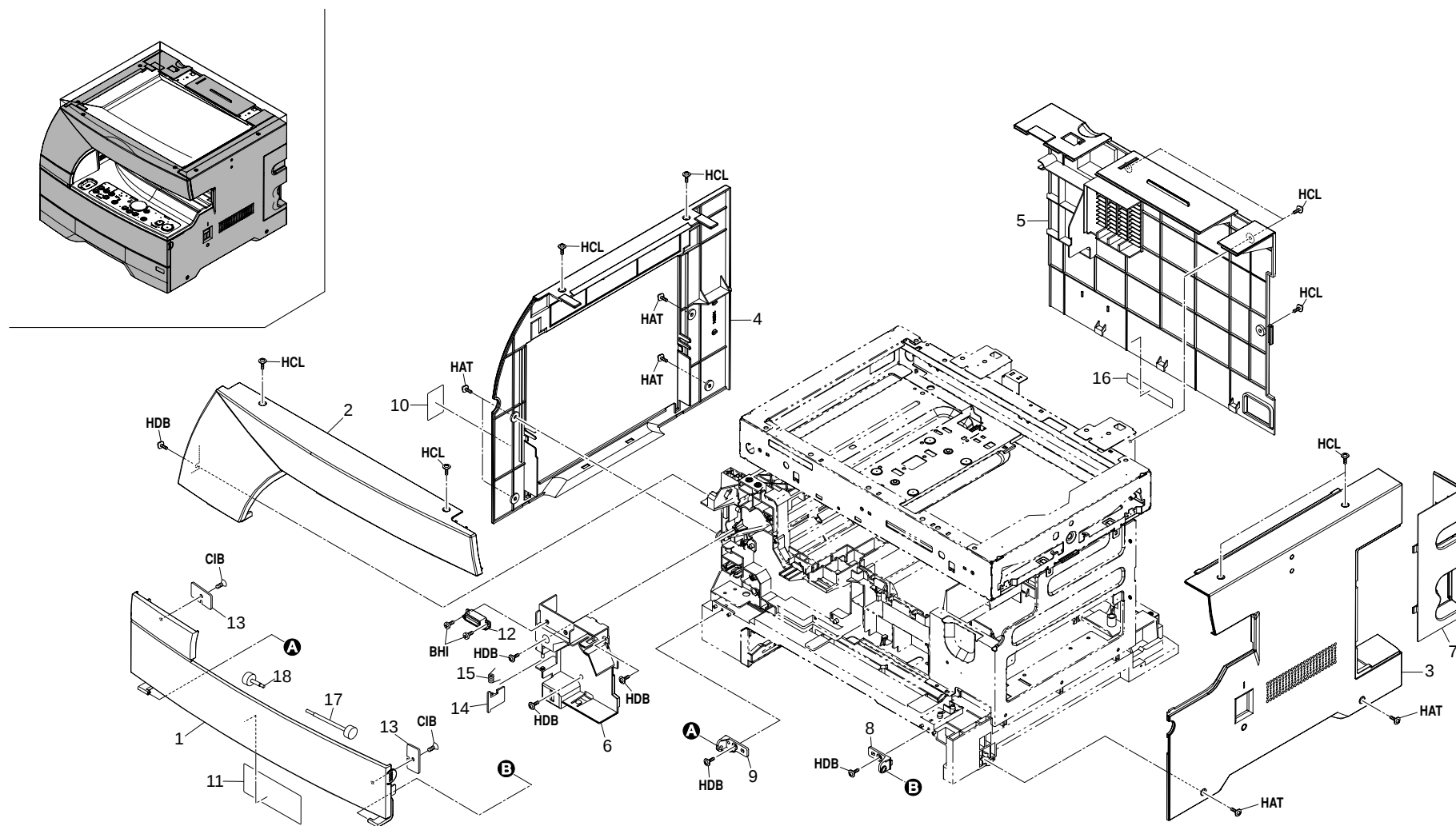
FIG. 1 EXTERIOR COVERS
