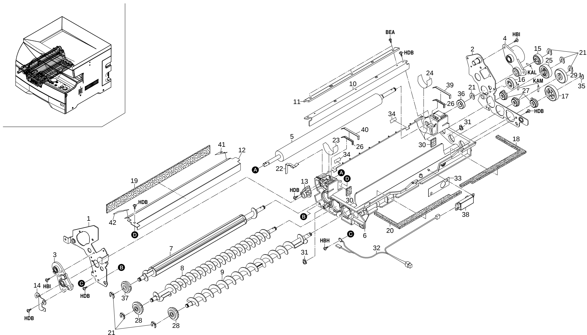
FIG. 8 IMAGING UNIT (DEVELOPING SECTION)
